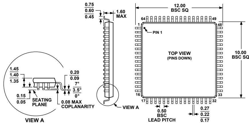
Figure 36. 64-Lead Low Profile Quad Flat Package [LQFP] (ST-64-2)
